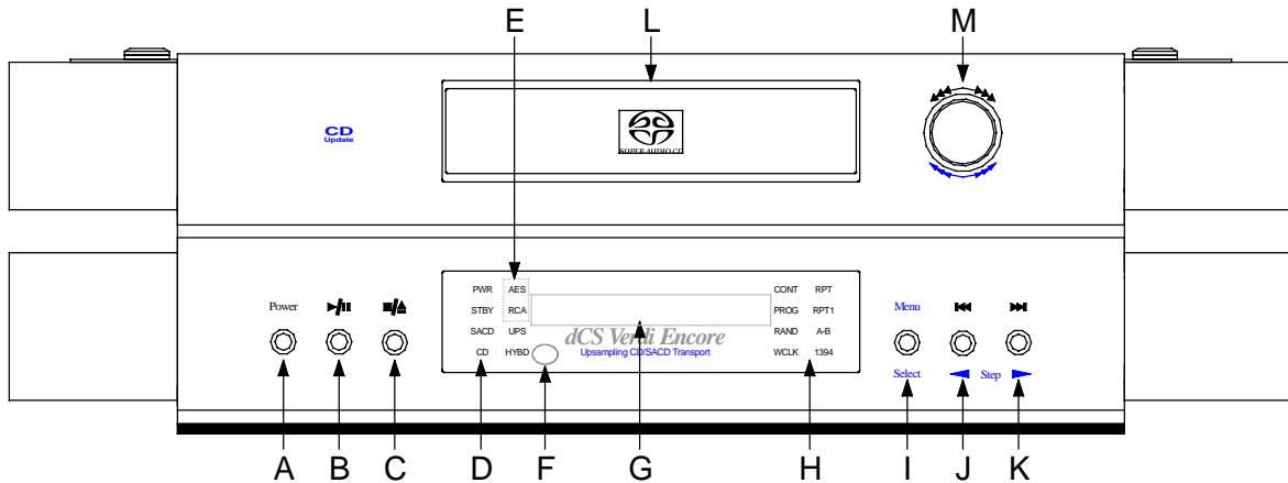
Figure 4 – dCS Encore Front Panel
