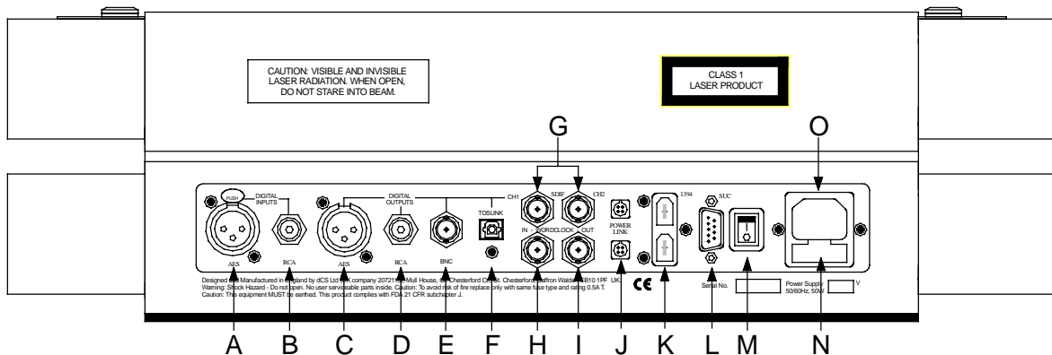
Figure 5 – dCS Verdi Encore Rear Panel
